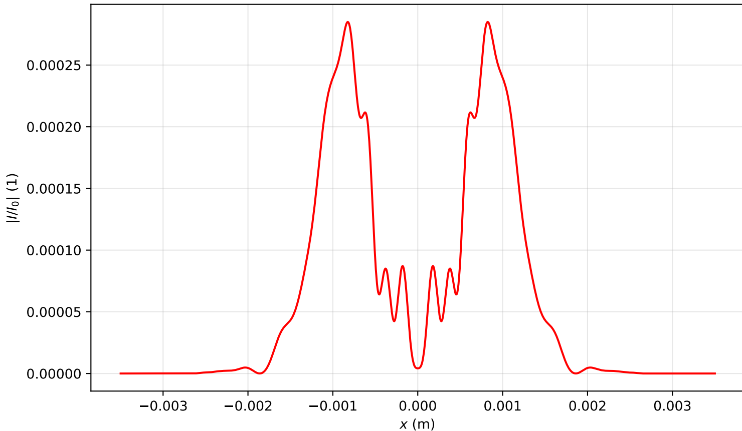
Intensity profile I(x, y = 0, z = 1.194)/I_0 , P_{in}=7.0P_{cr} , artificial time
